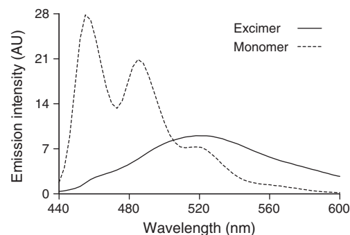
Fig. 6. Deconvoluted excimer and monomer spectra of perylene-daptomycin on DMPC/DMPG membranes. The steps involved in the deconvolution are described in the Materials and methods section.
