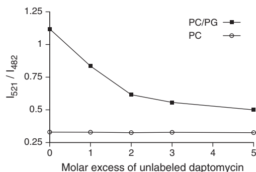
Fig. 5. Effect of unlabeled daptomycin on the extent of excimer formation by perylene-daptomycin. Perylene-daptomycin ( 2.5 \mu\text{M} ) was mixed with unlabeled daptomycin at the molar ratios indicated and incubated with DMPC/DMPG or DMPC liposomes with 6 and 200 mM of calcium, respectively. The change in fluorescence is represented the ratio of emission at 521 nm over that at 482 nm; a higher ratio indicates a greater extent of excimer formation.
