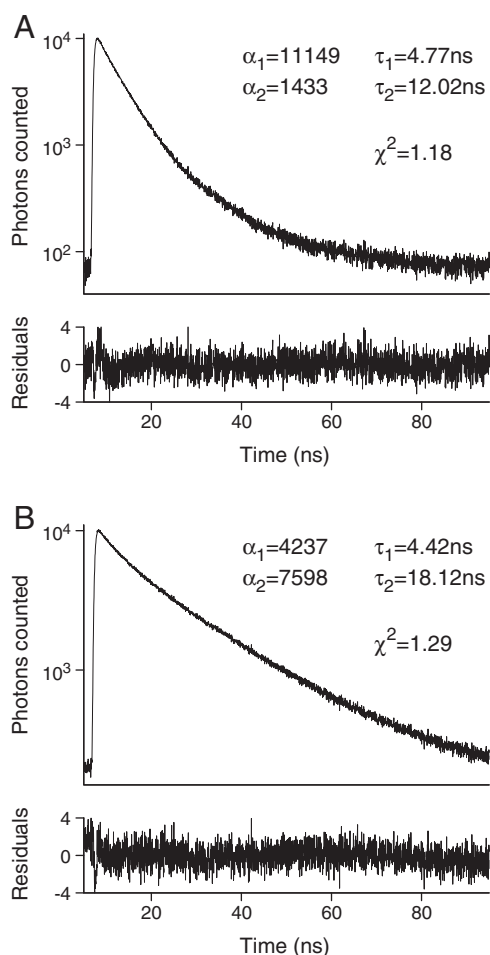
Fig. 4. Time-resolved fluorescence measurements of perylene-daptomycin on DMPC (A) and DMPC/DMPG (B) membranes. Sample composition was as in Fig. 3B and C, respectively. Excitation was with a 440 nm diode laser. Emission was measured using a 560 \pm 10 nm bandpass filter. The decays were fitted to a two-exponential model. Pre-exponentials ( \alpha ) and lifetimes ( \tau ) of the fitted components, as well as the residuals and \chi^2 of the fits are given.
