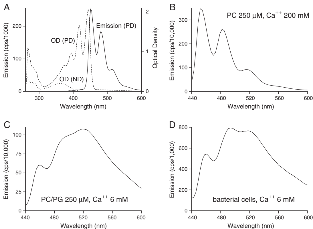
Fig. 3. Fluorescence emission spectra of perylene-daptomycin, in solution (A), on DMPC liposomes (B), on DMPC/DMPG liposomes (C), and on bacterial cells (D). The emission spectra were measured with 2.5 μM perylene-daptomycin. In (A), the absorption spectra of perylene-daptomycin (PD) and of native daptomycin (ND) at 50 μM in solution are also shown. The absorption spectrum of native daptomycin on membranes is indistinguishable (not shown). In (D), the cells were incubated with perylene-daptomycin and calcium, then washed twice by centrifugation to remove unbound daptomycin and resuspended before acquisition of the spectrum.
