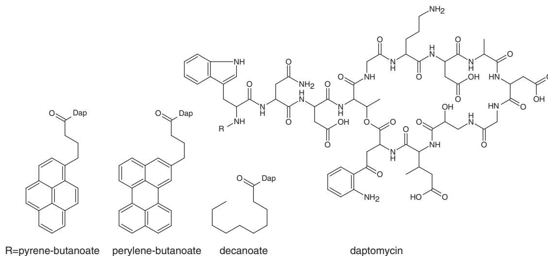
Fig. 1. Structure of daptomycin, and of the substituents pyrene- and perylene-butanoic acid that was substituted for the decanoyl residue of the native compound in this study.
