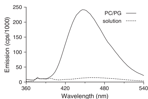
Fig. 2. Fluorescence emission spectra of pyrene-daptomycin in solution and on DMPC/DMPG liposomes, in the presence of 6 mM calcium. The excitation wavelength was 340 nm.
